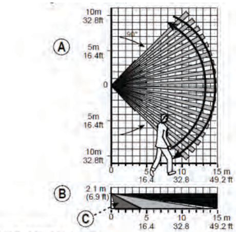
A. HORIZONTAL VIEW B. VERTICAL VIEW C. PG9904P: 2-4m (6.5 – 13ft)
